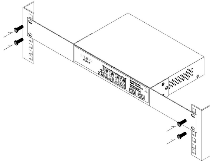
The SFC400GM, SFC450R Rack Mounting Diagram
